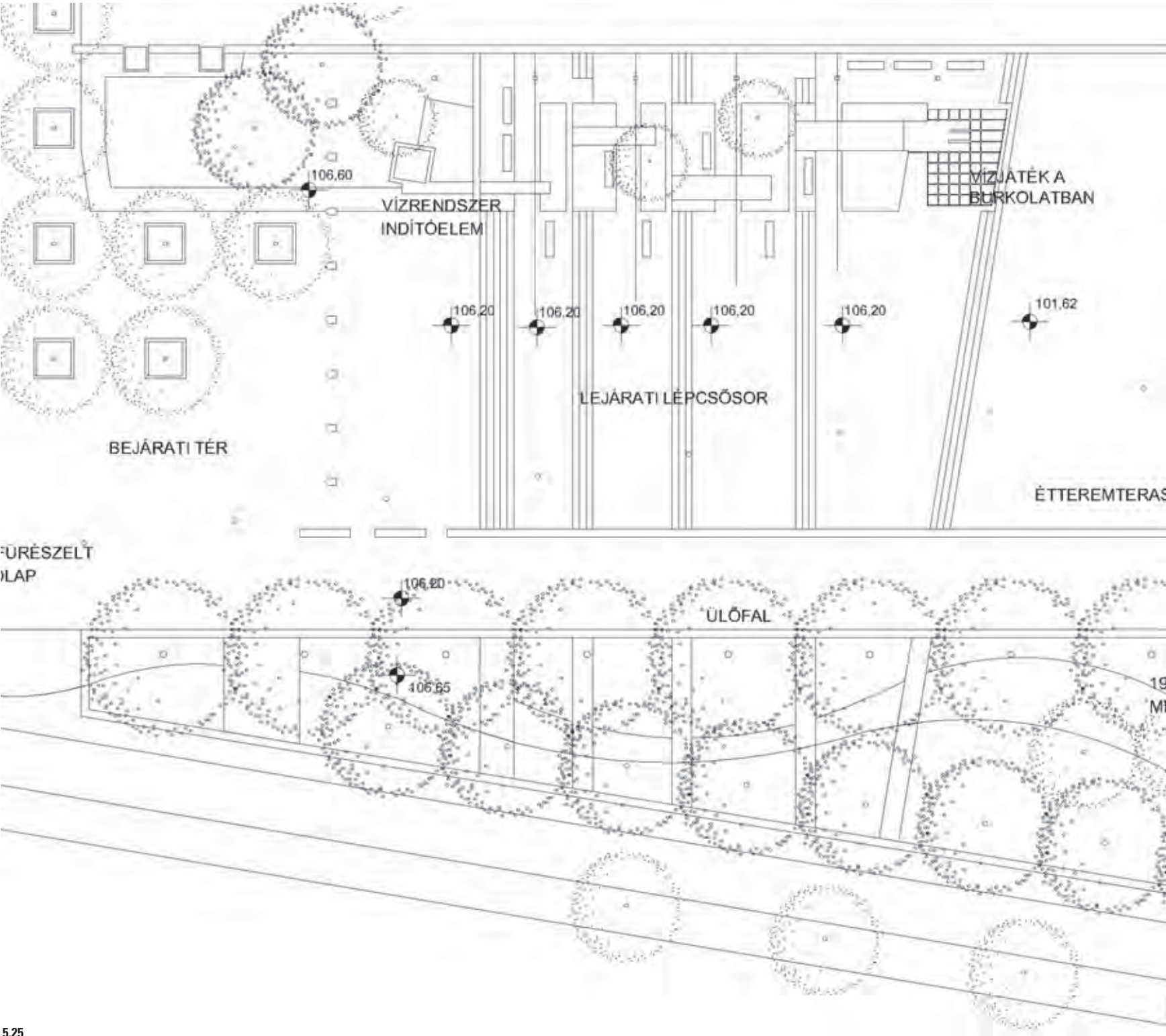
5.25 Plan of the Pool and the steps down to the Hole
