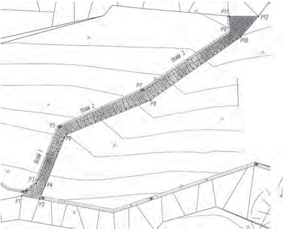
7.17 Plan of main path showing expansion joint positions. 'As built' plan
